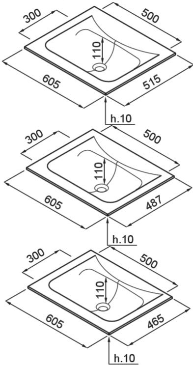
Technical Drawing
